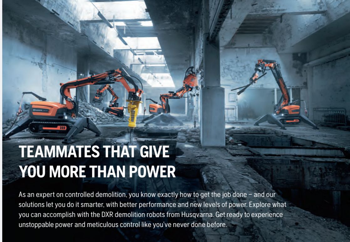
HYDRAULIC-POWERED HUSQVARNA DXR 95 9.8 kW, 589 kg, reach 3.2/2.7 m up/forward incl. tool.
